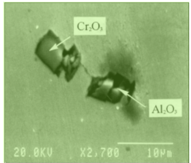
FIGURE 6. SEM micrograph of common oxides in type 444 SS after corrosion initiation but not propagation. 12
