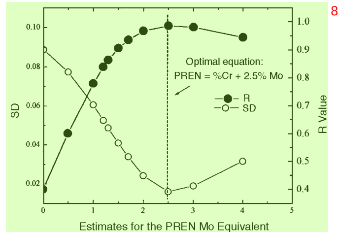
FIGURE 16. Estimates for the PREN molybdenum equivalent weighting factor in intermediate-chromium ferritic SS.
