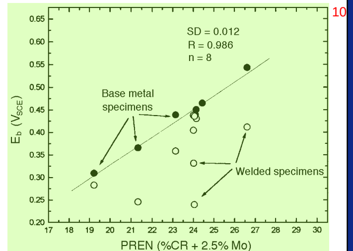
FIGURE 17. Summary of E_b of parent metal and welded, polished specimens as a function of variable PREN ( PREN = \%Cr + 2.5\% Mo ).
