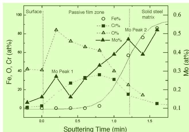
FIGURE 4. XPS depth profile of a ferritic SS containing 3% Mo. 10
