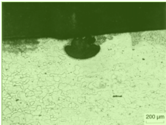
FIGURE 11. Optical micrograph of pit transverse section in a 18% Cr-2% Mo ferritic SS weld.
